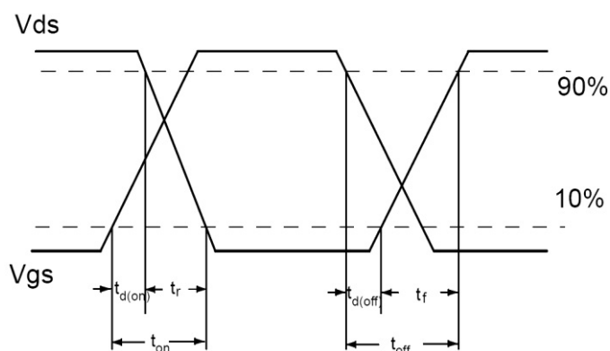
Switching Waveforms:
