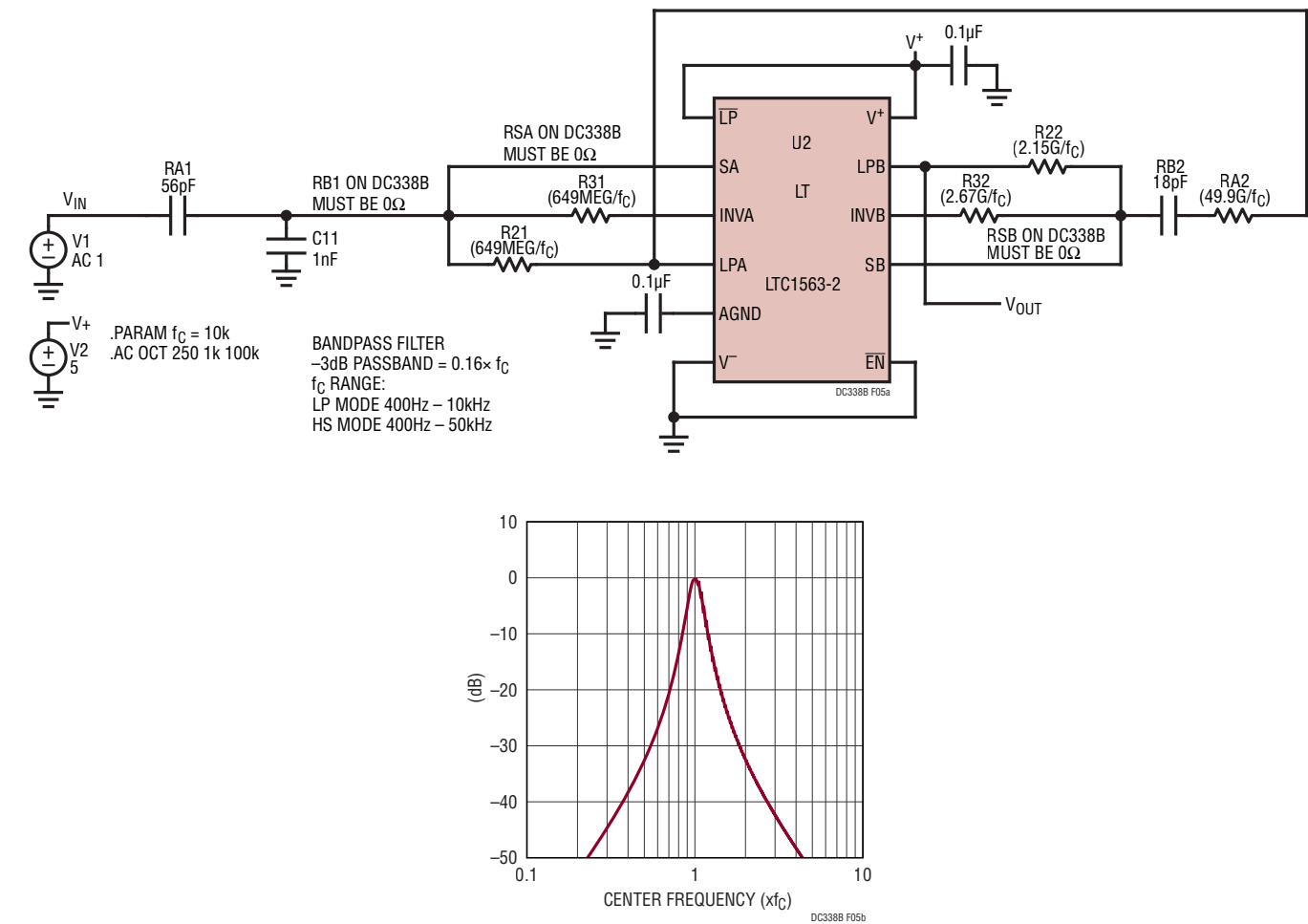
Figure 5. 4th Order Narrow Bandpass Filter
