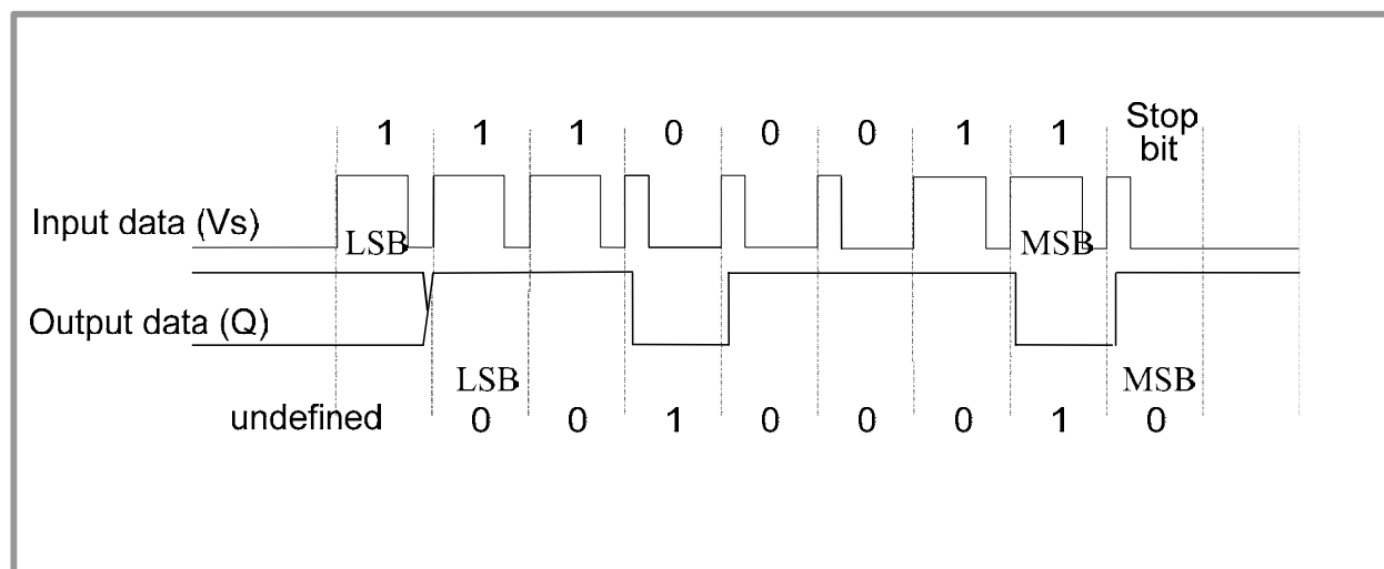
Fig. 5: Serial protocol
