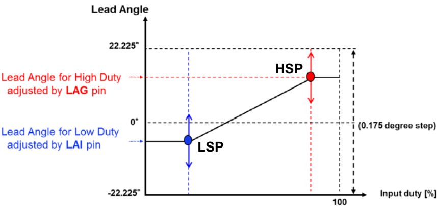
Figure 28. Image of Lead Angle Setting Curve
