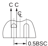
TOP VIEW 3.00BSC 2.75BSC 16 1 2 3 4 0.50 DIA 2.75BSC 3.00BSC 0.85 +0.15/-0.65 0.65 +0.15/-0.65 0.01 +0.04/-0.01 0.20 REF. 12° max SEATING PLANE BOTTOM VIEW 0.42 +0.18/-0.18 0.23 +0.07/-0.05 1.60 +0.10/-0.10 PIN 1 ID N 1 2 3 4 1.60 +0.10/-0.10 0.42 +0.18/-0.18 0.5 BSC 1.5 REF 0.40 +0.05/-0.05
