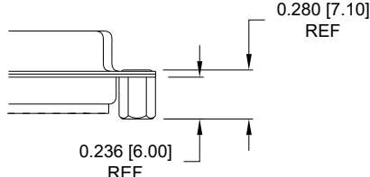
02 ..... 0.236" BOARD SIDE
