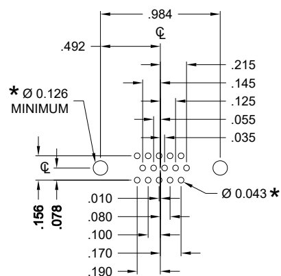
15 POSITION
