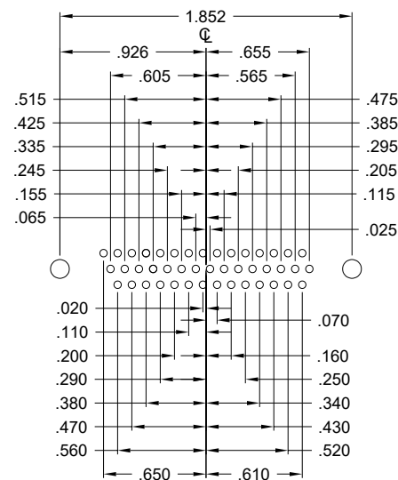
44 POSITION
