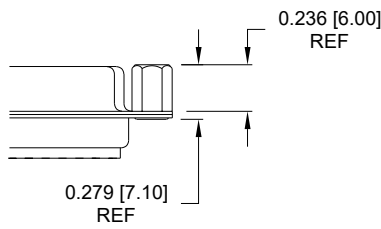
03 ..... 0.236" MATING SIDE
