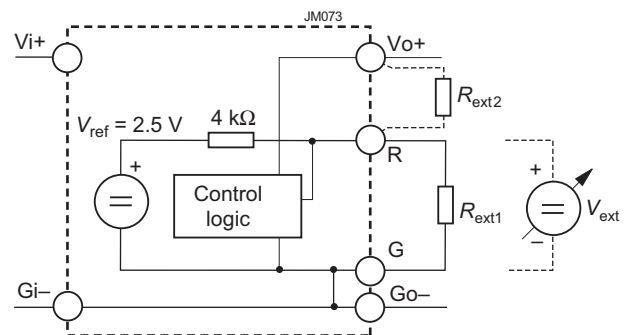
Fig. 10 Output voltage adjustment via R-input
