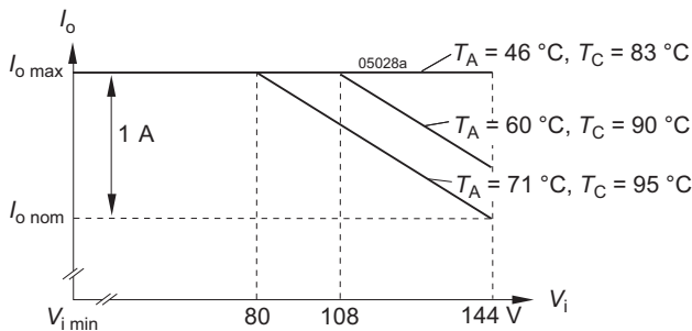
Fig. 5 Typ. dependance of I_{o\text{ L}} of temperature
