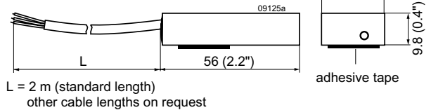
Fig. 15 Battery temperature sensor
