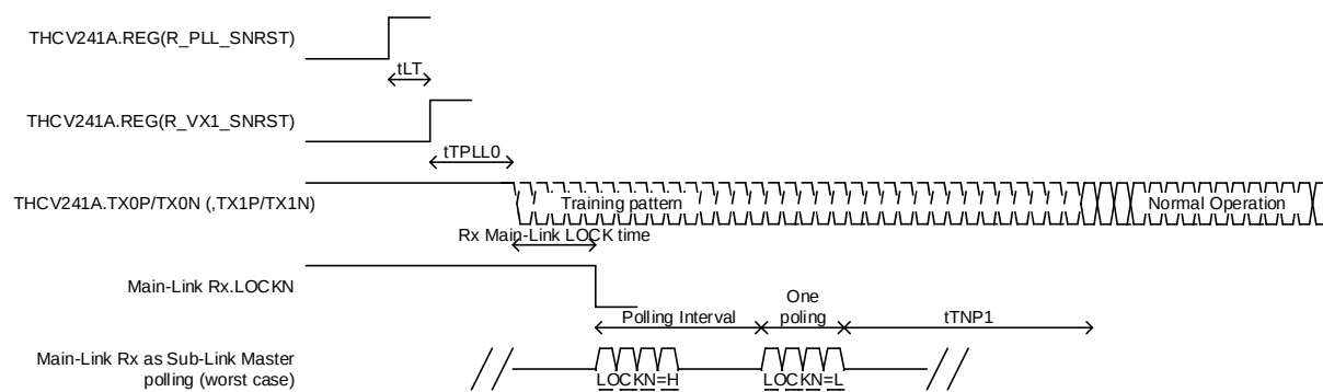
Figure 22. Lock Sequence
