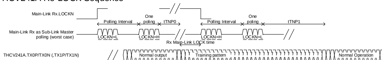
Figure 23. Re-Lock Sequence
