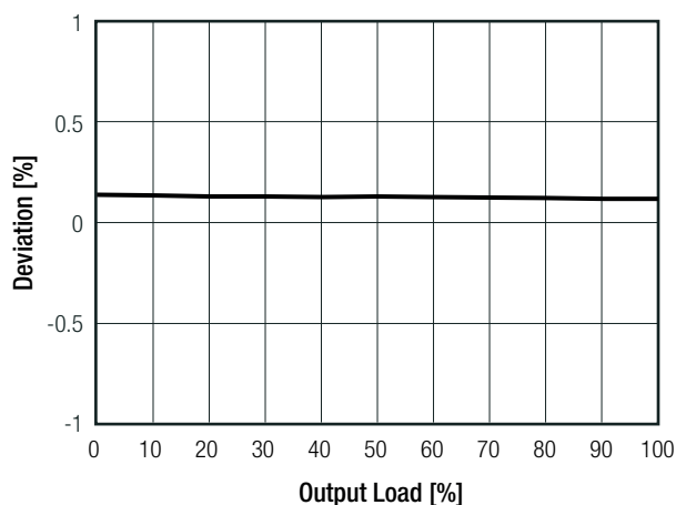
RAC05-12SK/277
