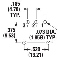
PC Mounting
