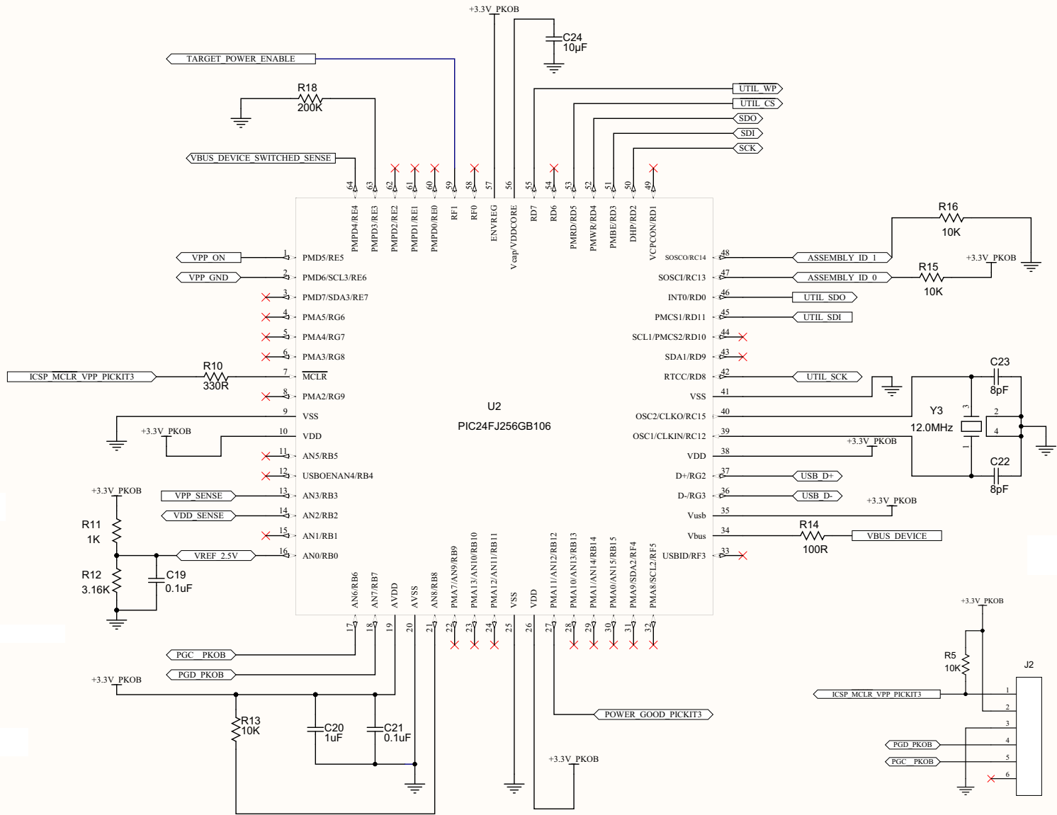
FIGURE A-8: DEBUGGER PIC24FJ256GB106 DEVICE
