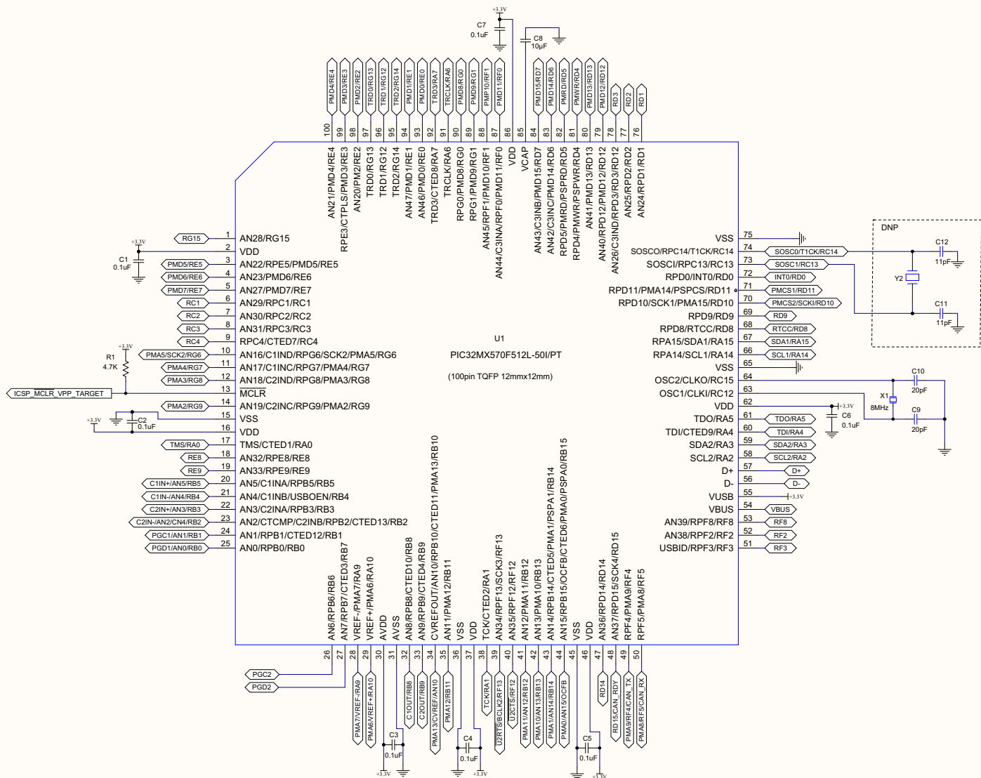
FIGURE A-2: PIC32MX570F512L (ON-BOARD DEVICE)
