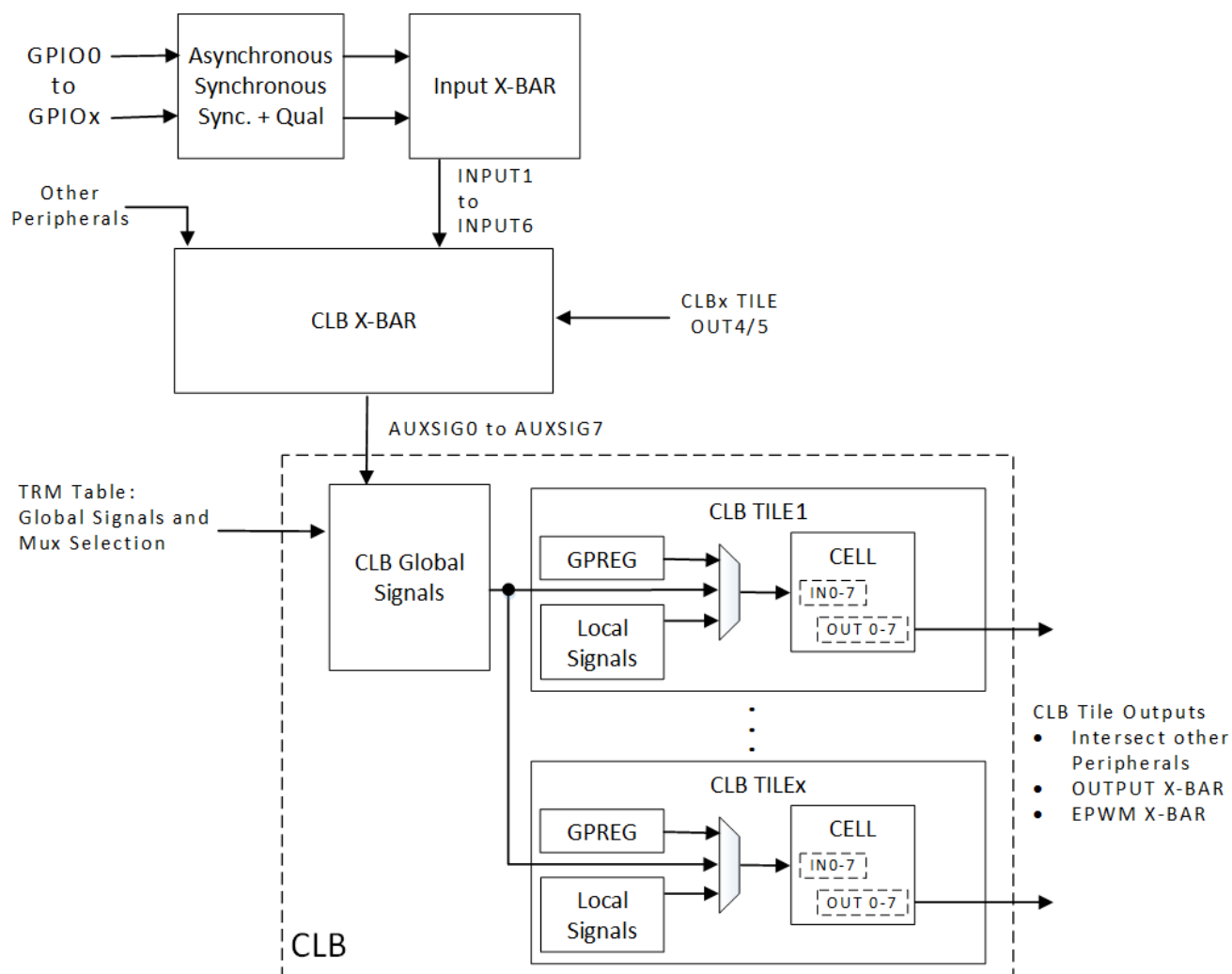
Figure 7-4. CLB Overview
