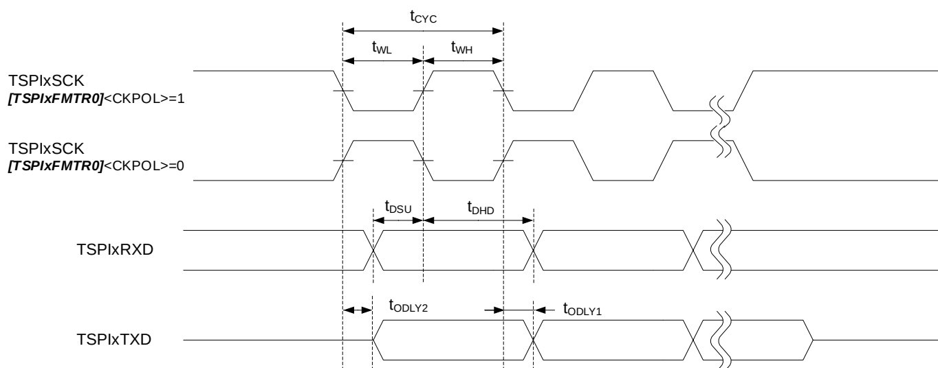
Figure 7.6 2nd Clock Edge Sampling (Target)
