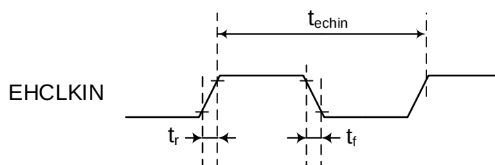
Figure 7.14 External Clock Input Waveform
