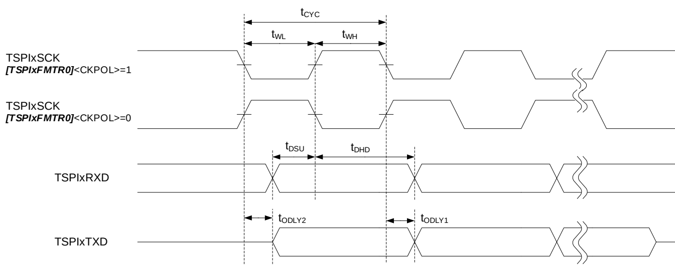
Figure 7.4 2nd Clock Edge Sampling (Controller)
