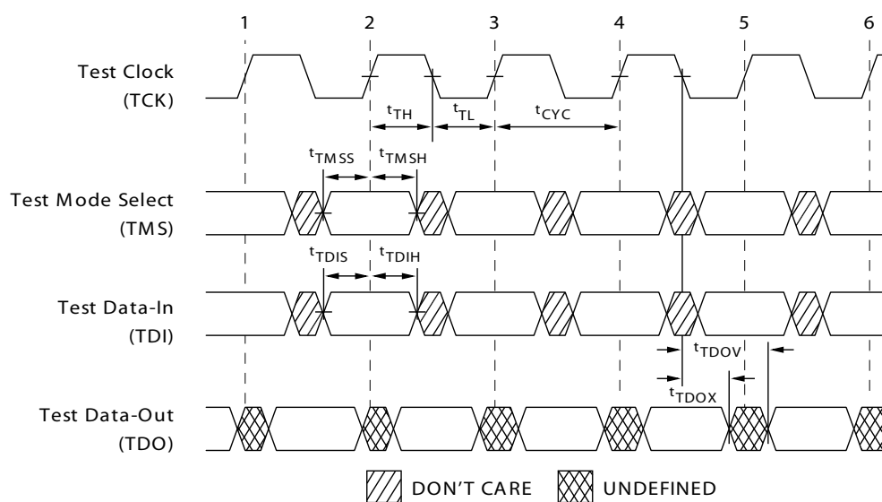
Figure 4. TAP Timing
