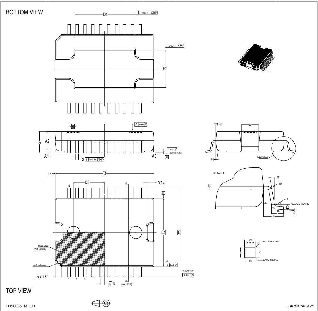
Figure 28. PowerSO-20 (slug-down) package mechanical drawing
