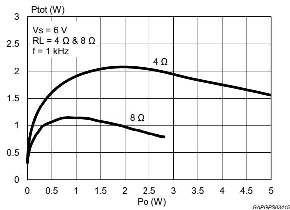
Figure 26. Power dissipation vs. output power ( R_L = 4\ \Omega & 8\ \Omega , sine, V_s = 6\text{ V} )
