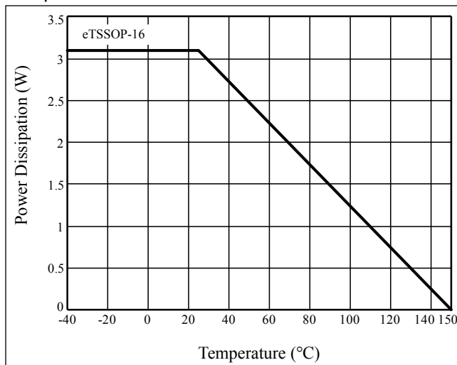
Figure 29 Dissipation Curve
