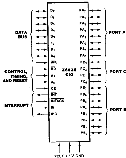
Figure 8-1. Z8536 (C10) Pin Functions
