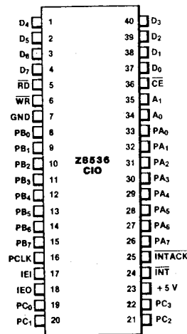
Figure 8-2. Z8536 (C10) Pin Assignments
