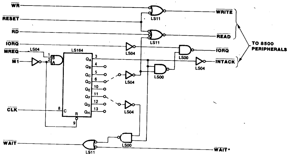
Figure 5-4. WAIT and INTACK Generation Logic
