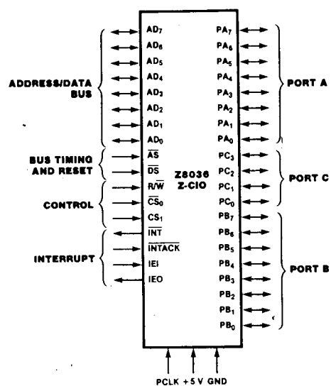
Figure 1. Pin Functions
