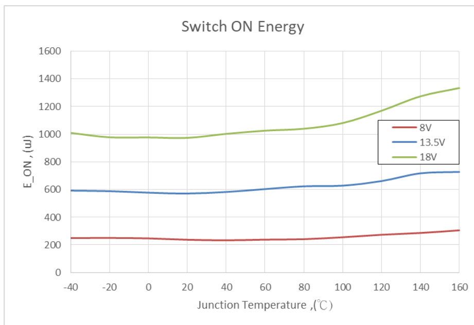
Figure 26. Switch ON Energy E_{ON} = f(T_J; V_S) , R_L=4\Omega .
