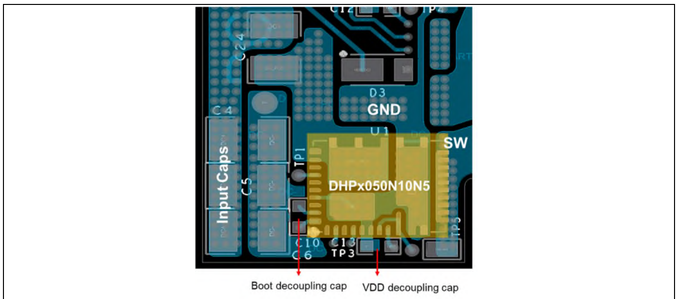
Figure 10 Example layout of DHPx050N10N5 in the primary side of a FB-FB 1/4 brick board - Top Layer
