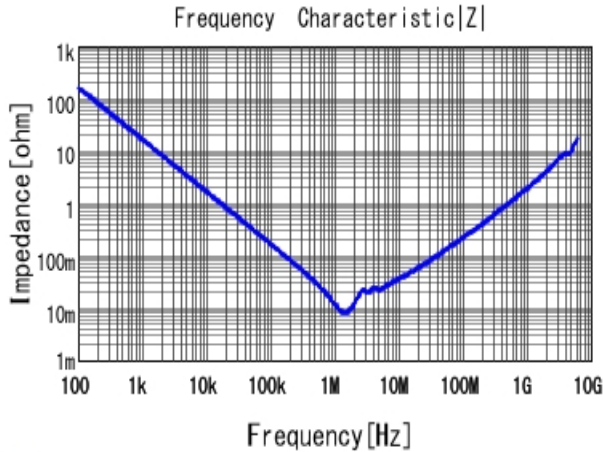
■ GRJ32EC71H106KE11 |Z| DC0V, 25degC
