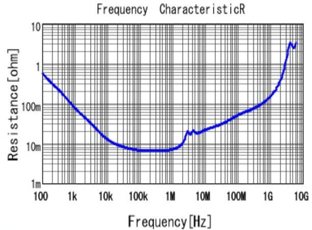
■ GRJ32EC71H106KE11 R DC0V, 25degC
