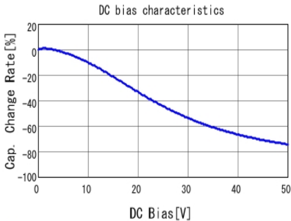
■ GRJ32EC71H106KE11 C-DC bias capchange, 25.0degC, AC1.
