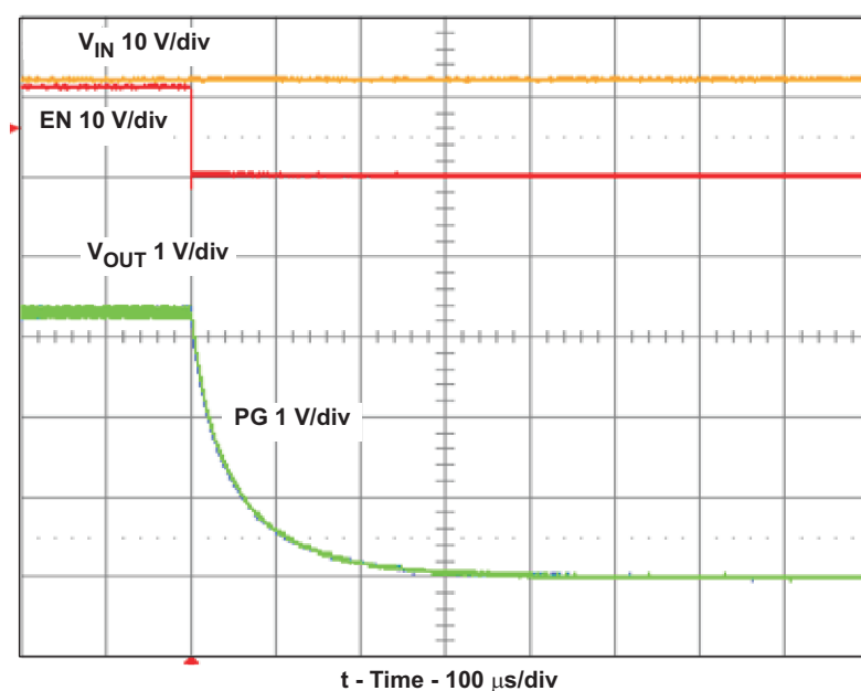
Figure 14. Shutdown on EN with 1-A Load and V_{IN} = 12 V
