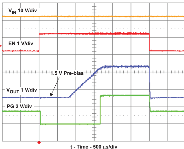
Figure 15. TLV62130 Prebias Start-Up and Shutdown on EN With 1-A Load and V_{\text{IN}} = 12\text{ V}
