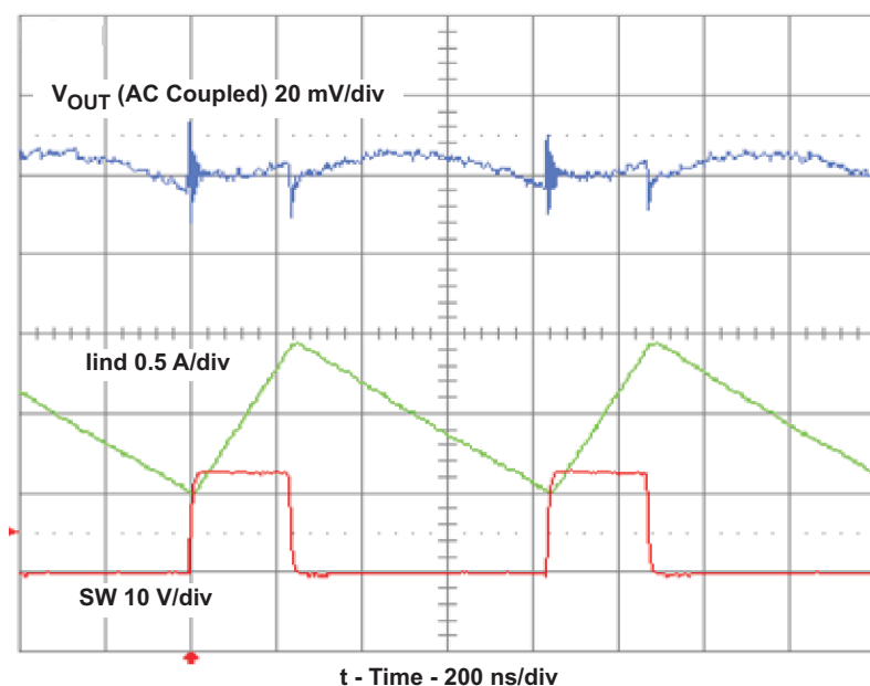
Figure 10. Output Voltage Ripple With 2.2-μH Inductor and FSW = HIGH (Low Frequency) and V_{IN} = 12 V and I_{OUT} = 1 A
