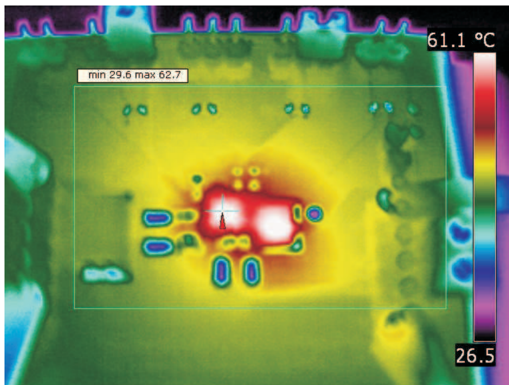
Figure 18. Thermal Performance With 2.2-μH Inductor
