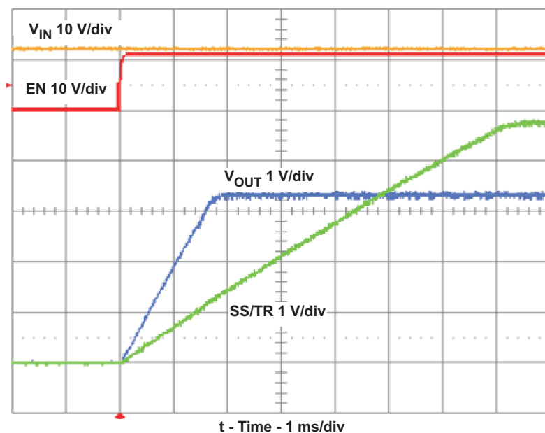
Figure 13. Start-Up on EN with 1-A Load and V_{IN} = 12 V
