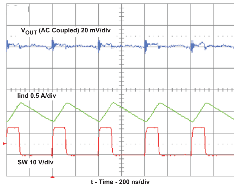
Figure 9. Output Voltage Ripple With 2.2-μH Inductor and FSW = LOW (High Frequency) and V_{IN} = 12 V and I_{OUT} = 1 A
