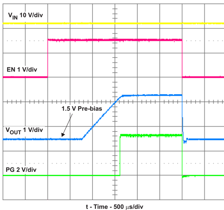
Figure 16. TLV62130A Prebias Start-Up and Shutdown on EN With 1-A Load and V_{\text{IN}} = 12\text{ V}
