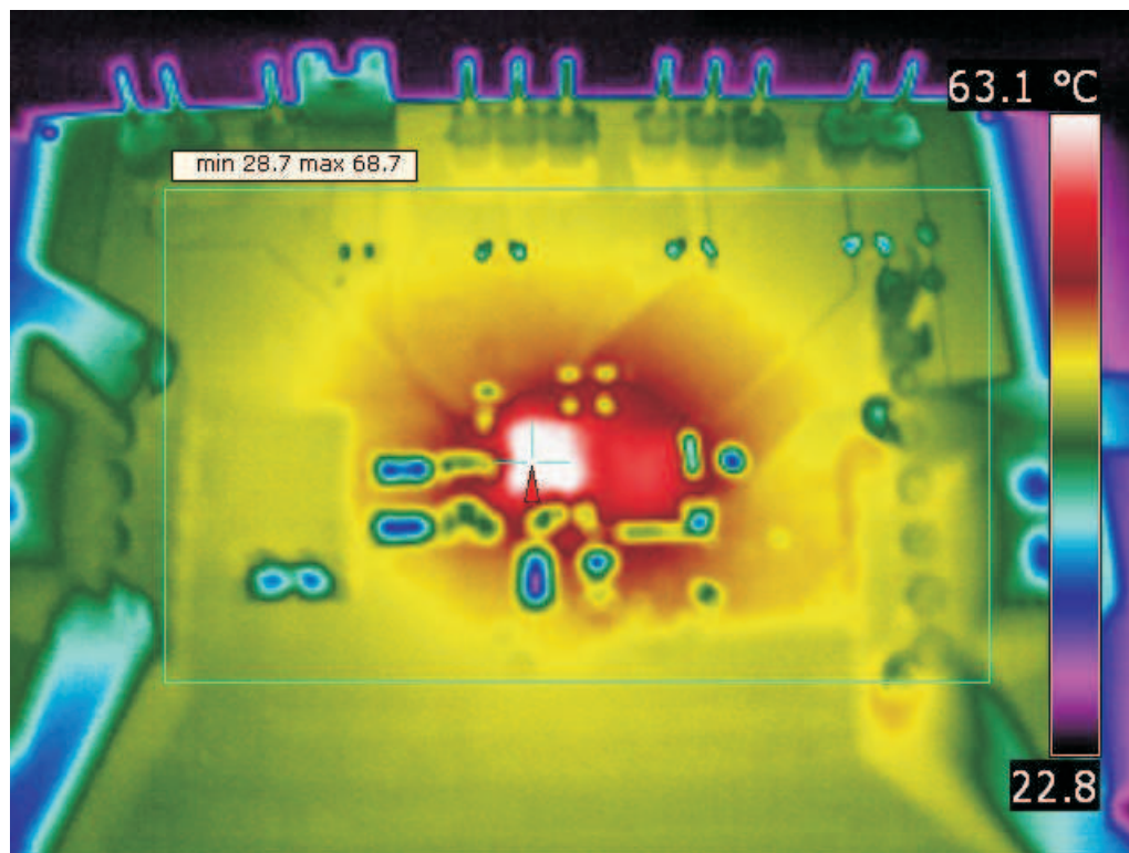
Figure 17. Thermal Performance With 1-μH Inductor
