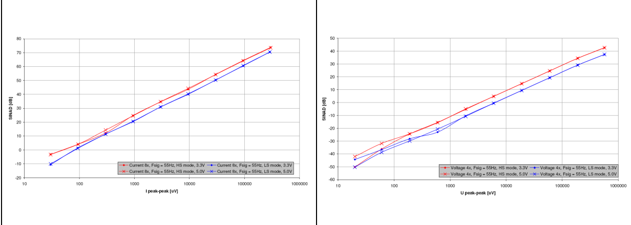
Figure 11. SINAD of CIP-CIN channel, gain 8x Figure 12. SINAD of VIP-VIN channel
