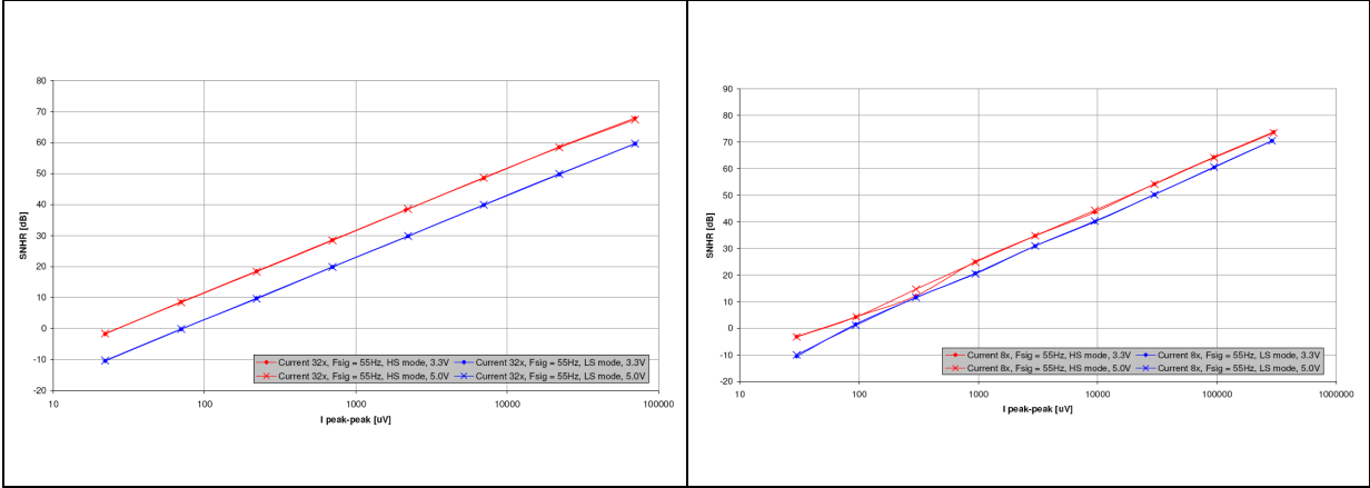
Figure 9. SNHR of VIP-VIN channel Figure 10. SINAD of CIP-CIN channel, gain 32x
