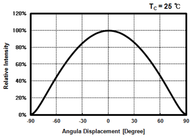
Radiation Pattern
