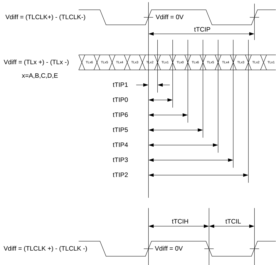
Figure 13 LVDS Input Switching Timing Diagrams
