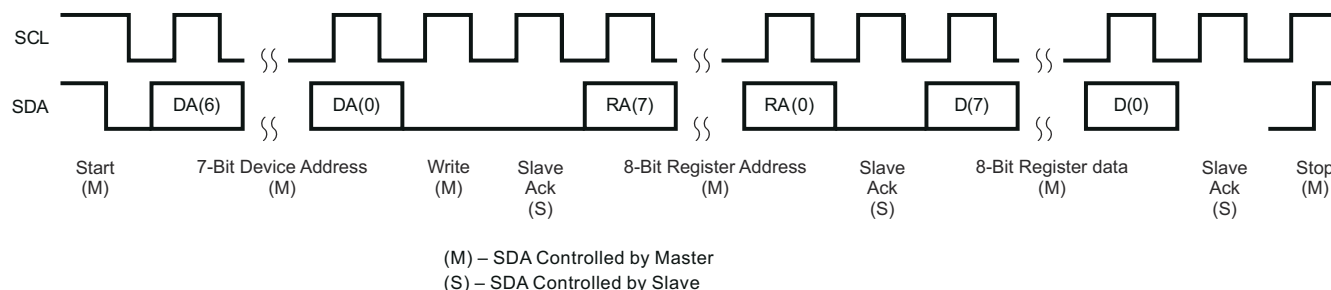
Figure 10-24. I²C Write
