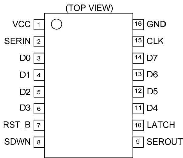
Figure 2. Pin Configuration
