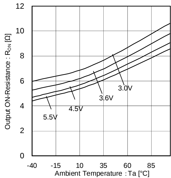
Figure 7. Output ON Resistance (Temperature characteristic @ I_D=20\text{mA} )
