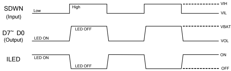
Figure 15. PWM Signal
