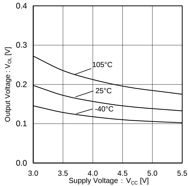
Figure 11. SEROUT Low Side Voltage ( V_{CC} characteristic @ I_{SO}=4mA )
