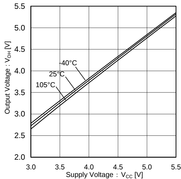
Figure 9. SEROUT High Side Voltage ( V_{CC} characteristic @ I_{SO}=-4mA )
