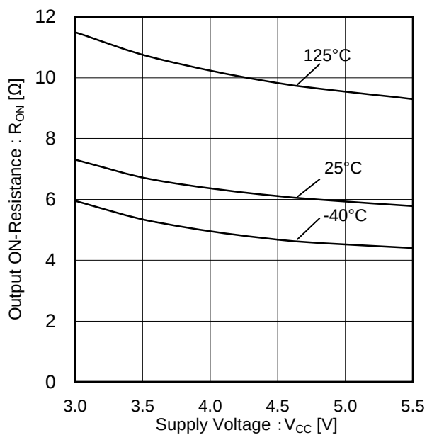
Figure 6. Output ON Resistance (VCC characteristic @ I_D=20\text{mA} )
