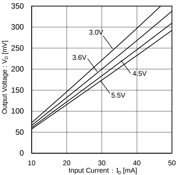
Figure 8. Output ON Resistance ( I_D characteristic)
