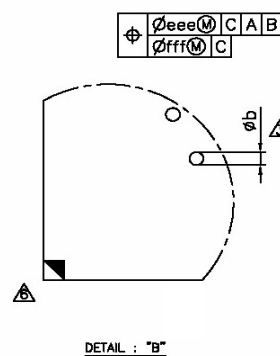
Figure 3- Package Outline Drawing – bottom view
