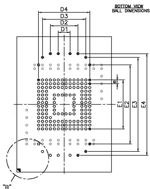
Figure 3- Package Outline Drawing – bottom view
