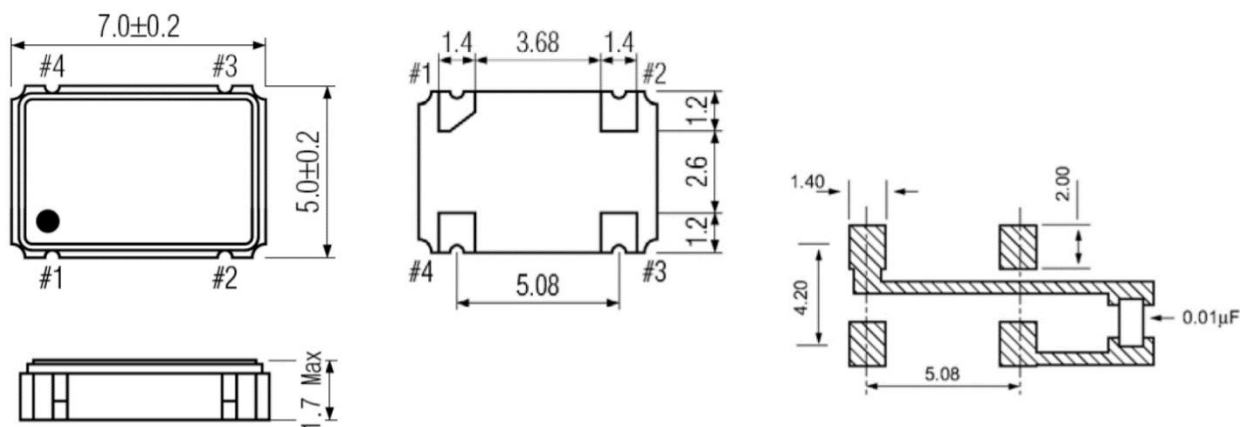
Figure 2) Land Pattern
