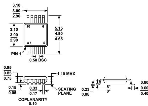
COMPLIANT TO JEDEC STANDARDS MO-187-BA Figure 38. 10-Lead Mini Small Outline Package [MSOP] (RM-10) Dimensions shown in millimeters
