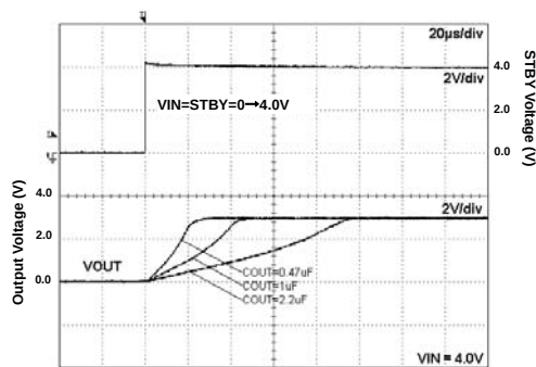
Fig 229. Start Up Time (VIN=STBY) Iout=0mA
