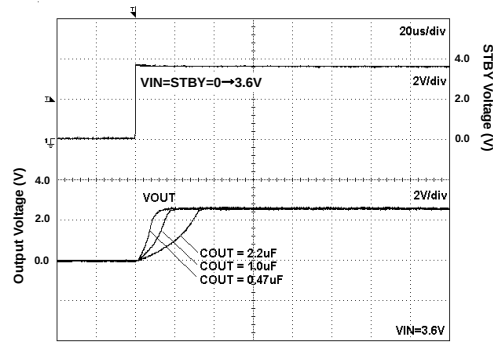
Fig 151. Start Up Time (VIN=STBY) Iout=0mA Iout=0mA
