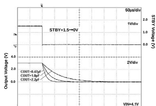
Fig 257. Discharge Time
