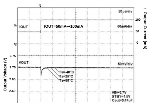
Fig 173. Load Response
