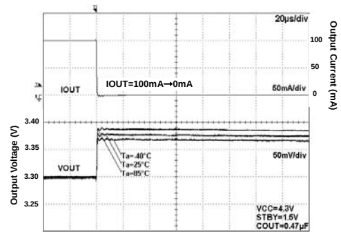
Fig 274. Load Response
