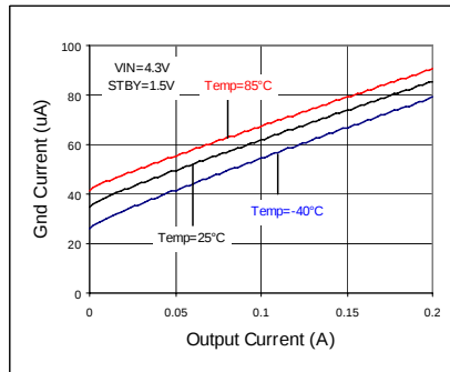
Fig 263. IOUT - IGND
