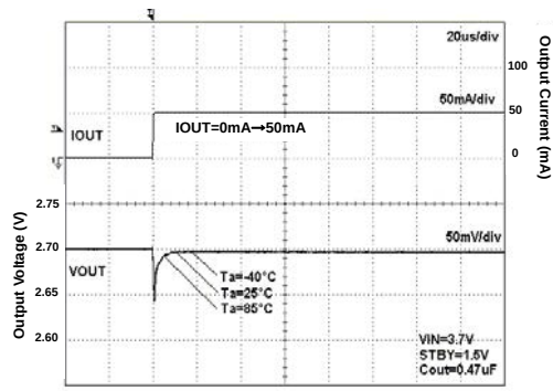
Fig 167. Load Response
