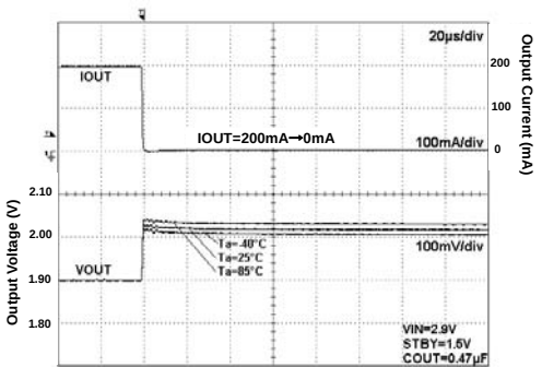
Fig 94. Load Response
