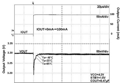
Fig 273. Load Response
