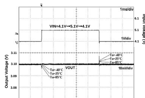
Fig 258. VIN Response
