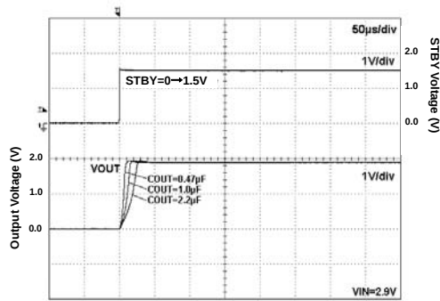
Fig 97. Start Up Time Iout=0mA
