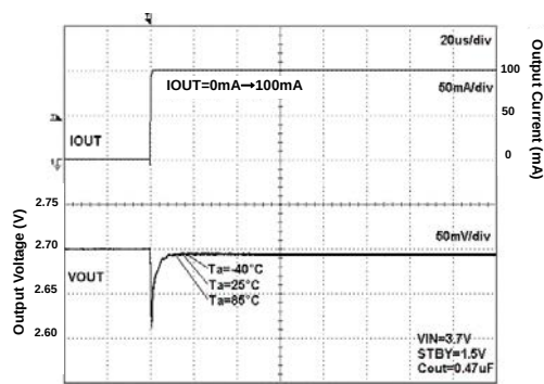
Fig 169. Load Response
