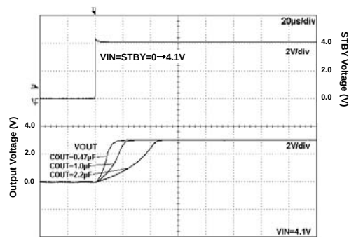
Fig 255. Start Up Time (VIN=STBY) Iout=0mA Iout=0mA
