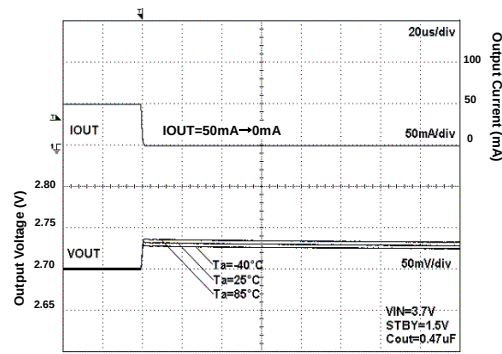
Fig 168. Load Response
