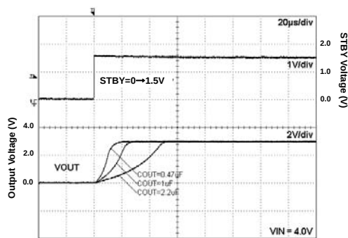
Fig 227. Start Up Time Iout=0mA
