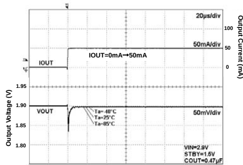
Fig 89. Load Response
