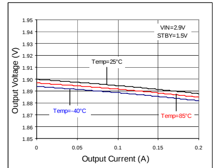
Fig 83. Load Regulation
