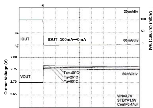
Fig 170. Load Response
