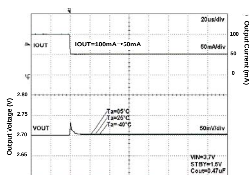
Fig 174. Load Response
