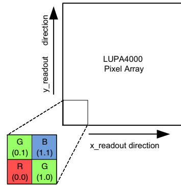
Figure 2. Color Filter Array
