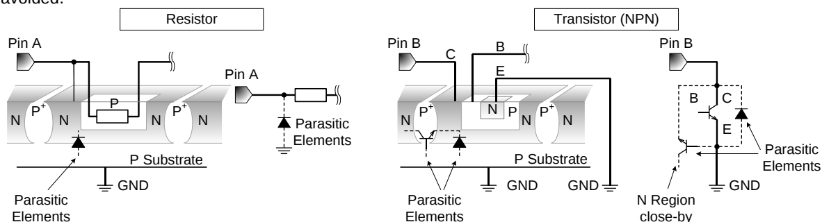
Figure 101. Example of monolithic IC structure
