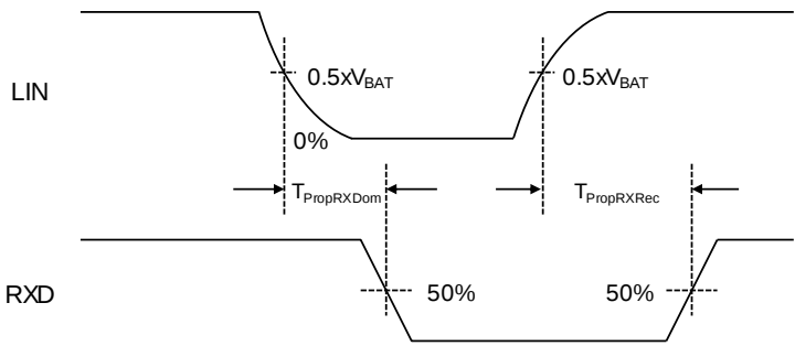
Figure 5. AC characteristic timing chart
