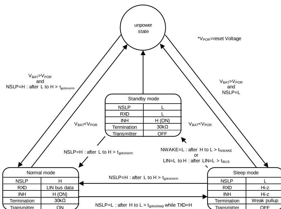
Figure 4. State Transition Chart
