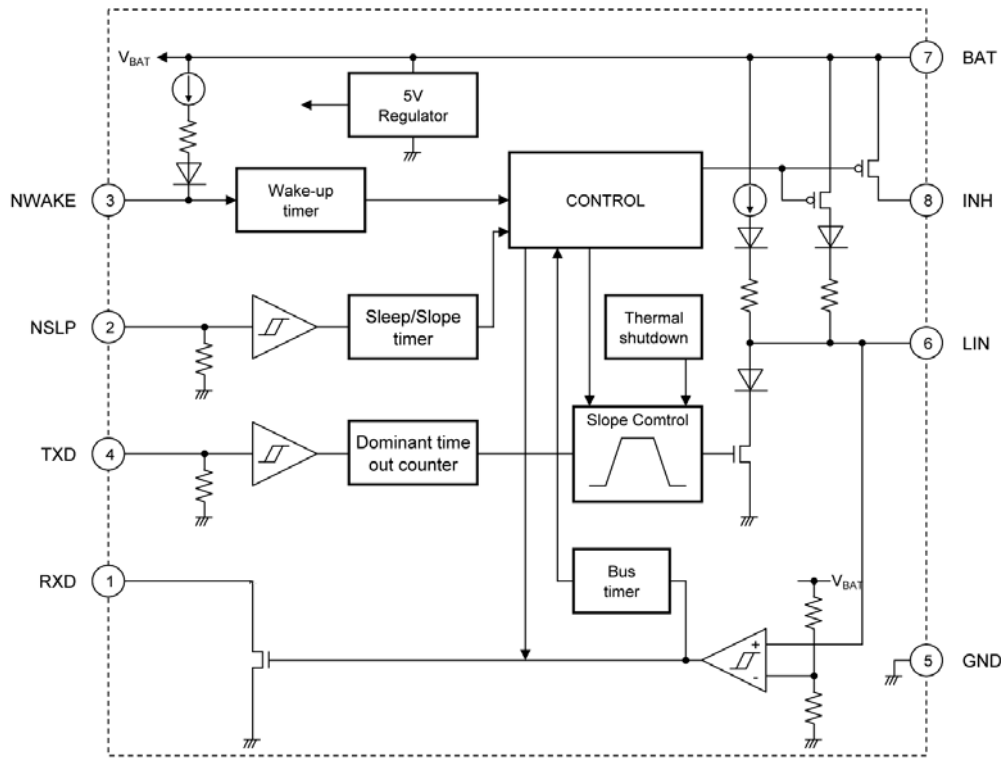
Figure 3. Block diagram
