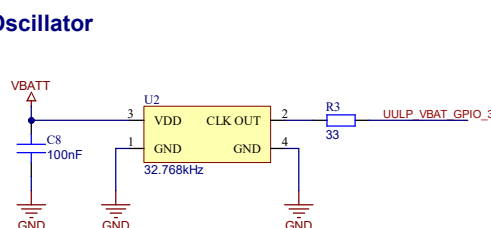
Figure 8.11. 32.768 kHz Clock Oscillator
