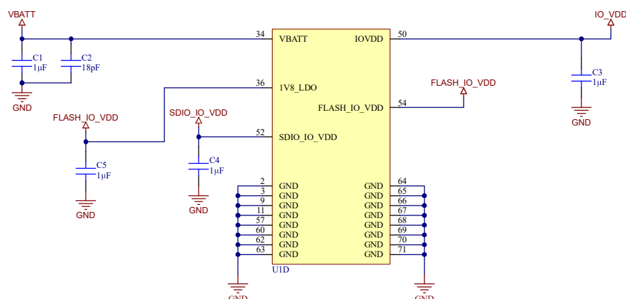
Figure 8.7. System Power Supplies
