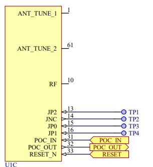
Figure 8.8. RF, Debug, and Reset Connection
