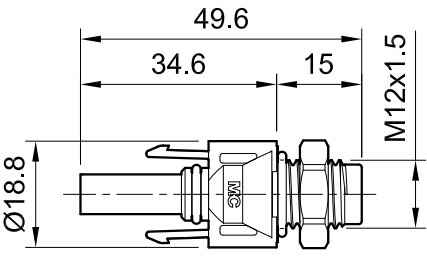
Female panel receptacle PV-ADBP4-S2...
