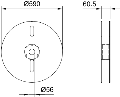
Reel with contacts
