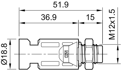
Male panel receptacle PV-ADSP4-S2...
