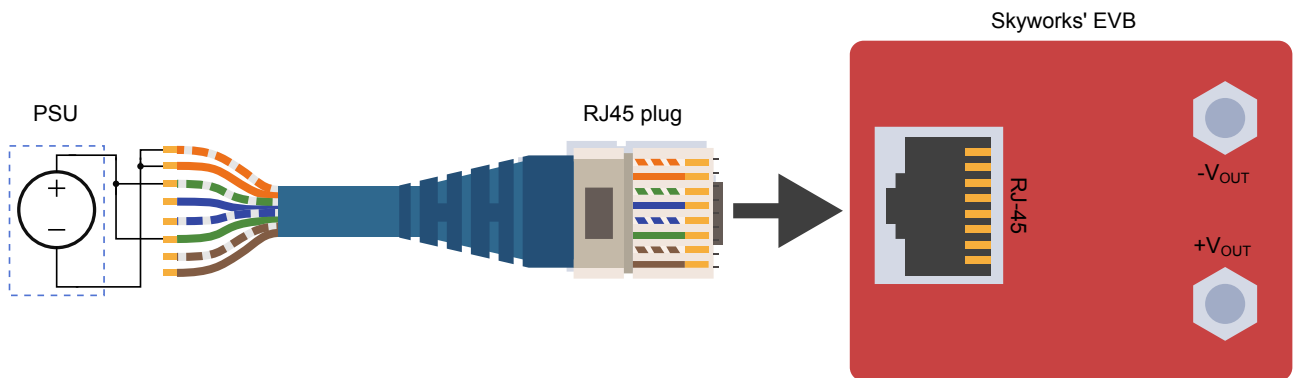
Figure 2.2. Midspan Connection using Laboratory Power Supply
