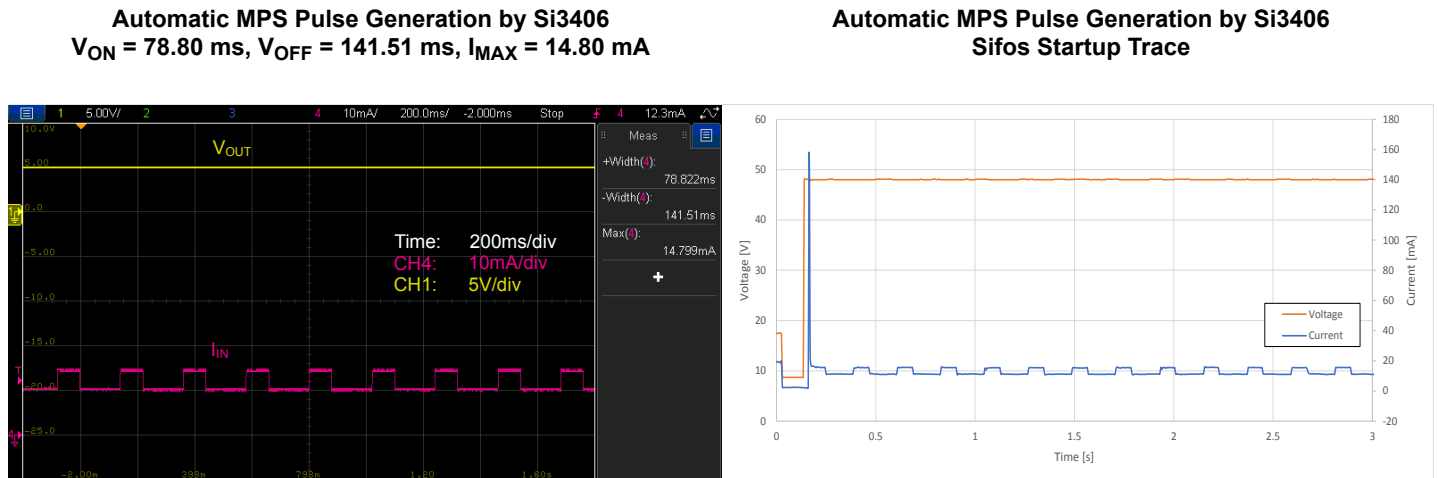
Figure 5.11. Si3406-Buck Non-Isolated EVB, 5 V, Class 2 PD Automatic Maintain Power Signature (MPS) Generation
