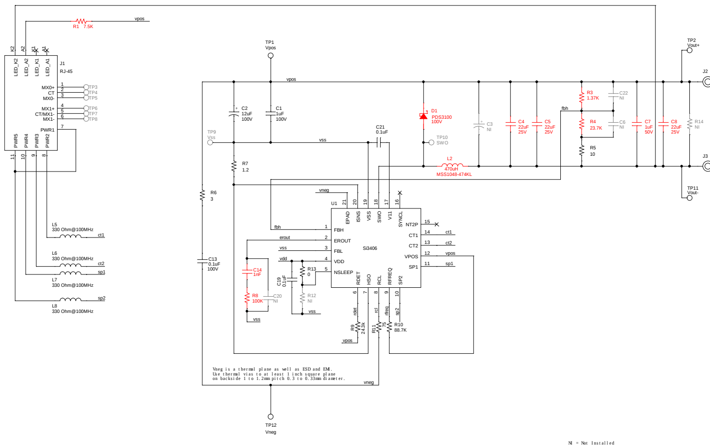
Figure 7.1. Si3406 Buck Non-Isolated EVB Schematic: 24 V, Class 2 PD
