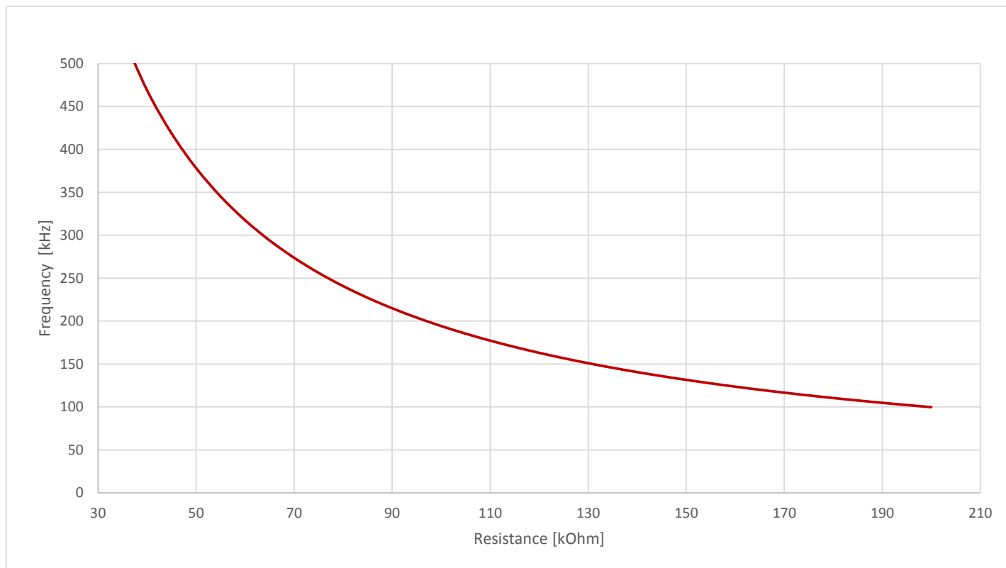
Figure 8.1. Switching Frequency vs R_{FREQ}
