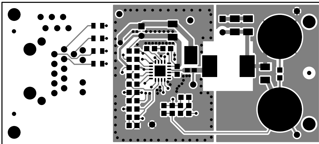
Figure 9.2. Top Layer
