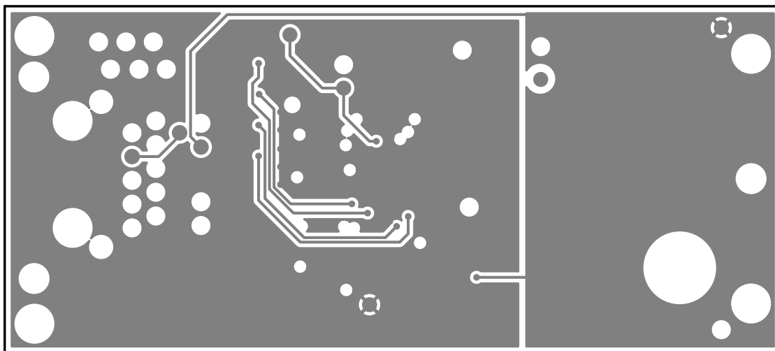
Figure 9.3. Internal 1 (Layer 2)
