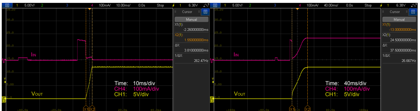
Figure 6.7. Si3406-Buck Non-Isolated EVB, 12 V, Class 2 Output Voltage Soft-Start at Low-Load (Left) and Heavy-Load (Right) Conditions
