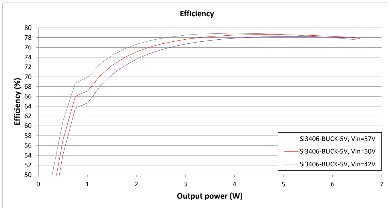
Figure 5.2. Si3406-Buck End-to-End Efficiency Chart with Internal Diodes as Input Bridge: 42 V, 50 V and 57V Input, 5 V Output, Class 2
