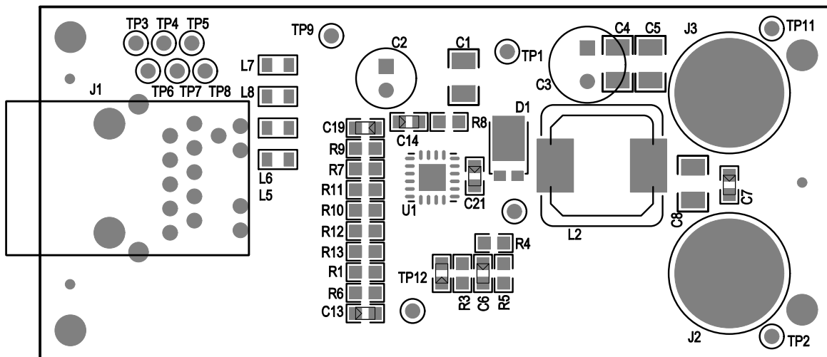
Figure 9.1. Top Silkscreen
