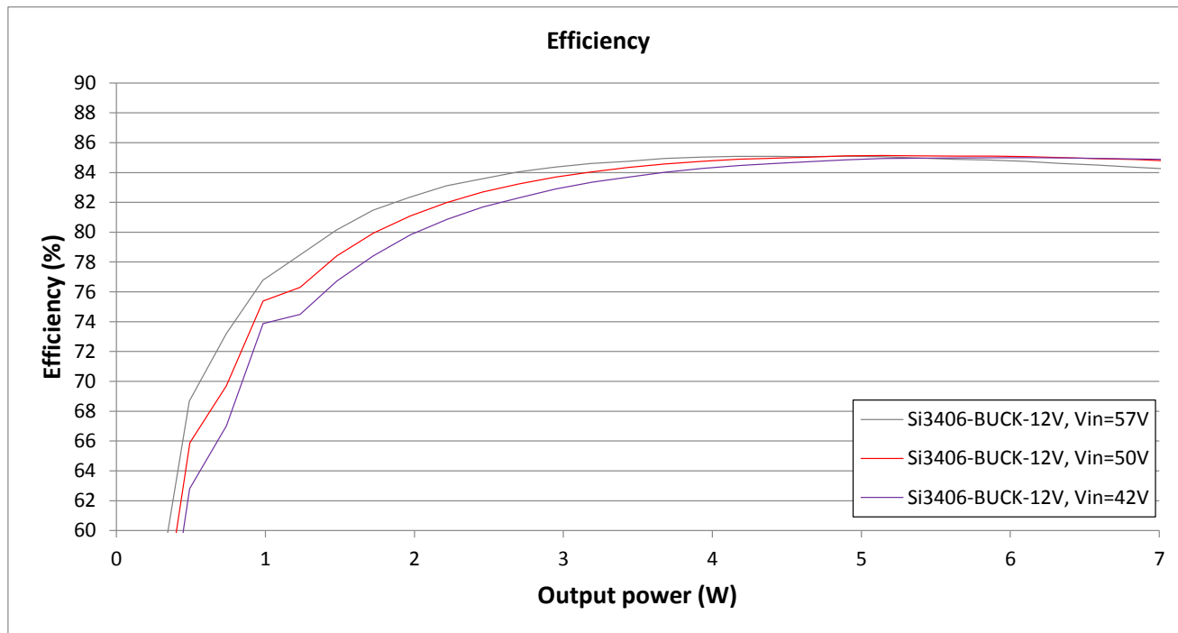
Figure 6.2. Si3406-Buck End-to-End Efficiency Chart with internal Diodes as Input Bridge: 42V, 50 V and 57V Input, 12 V Output, Class 2
