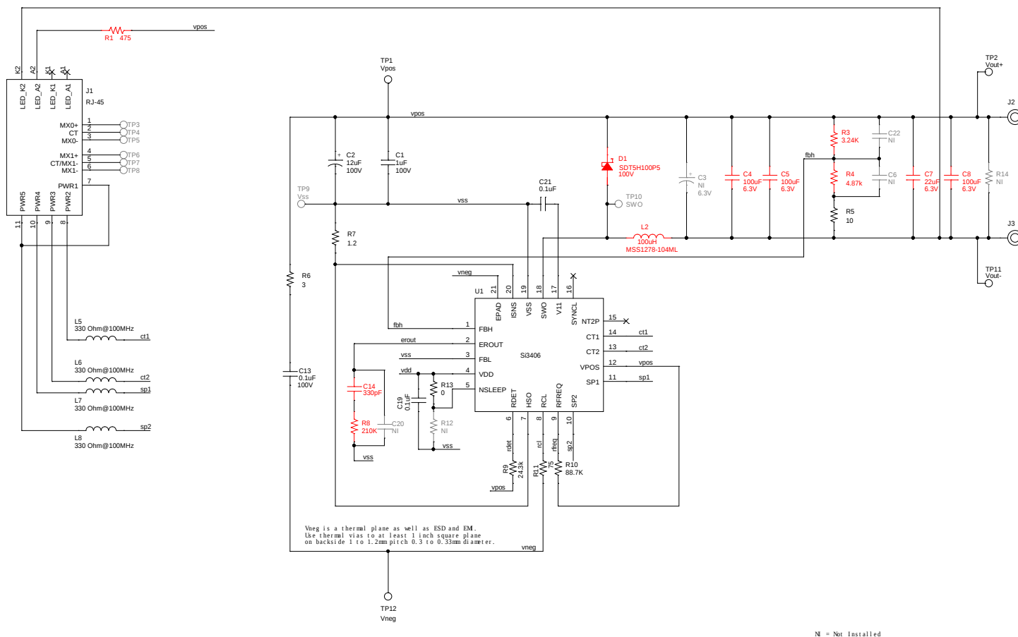
Figure 4.1. Si3406 Buck Non-Isolated EVB Schematic: 3.3 V, Class 2 PD, 7 W
