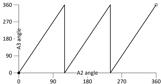
Figure 10: Angle gain behavior over full rotation with gain = 3 and ANG_GAIN_SAT_EN = 0
