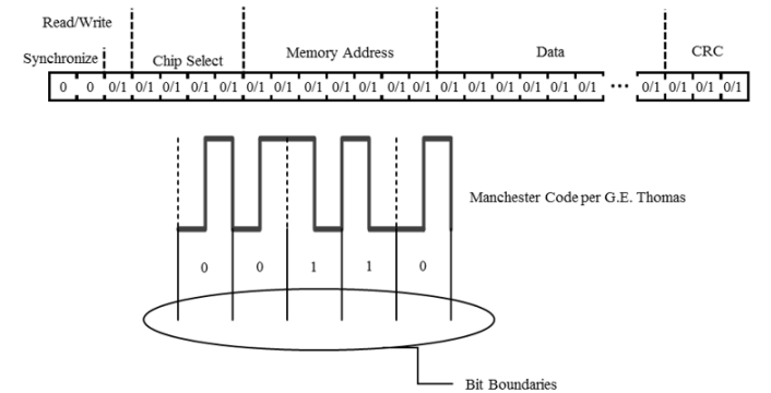
Figure 27: Manchester Bit Stream Definition
