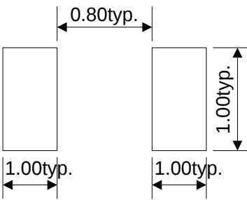
Recommended Pad Layout (mm)
