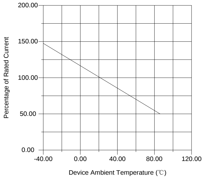
Recommended Hold Current (A) at Ambient Temperature (°C)
