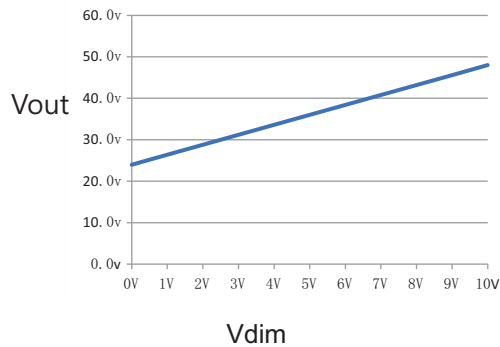
Dimming Curve
