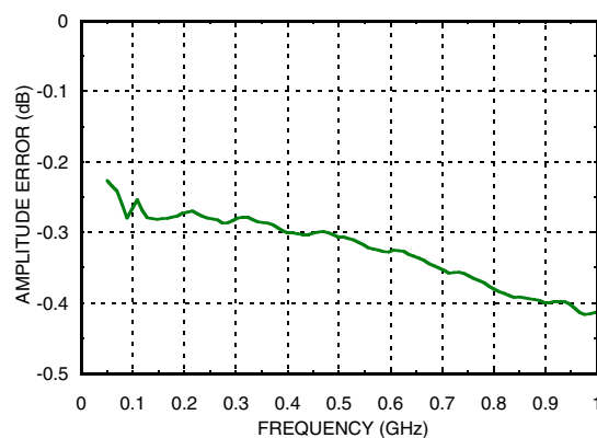
Amplitude Balance *
