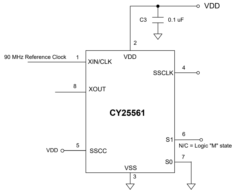
Figure 4. Application Schematic
