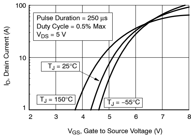
Figure 3. Transfer Characteristic
