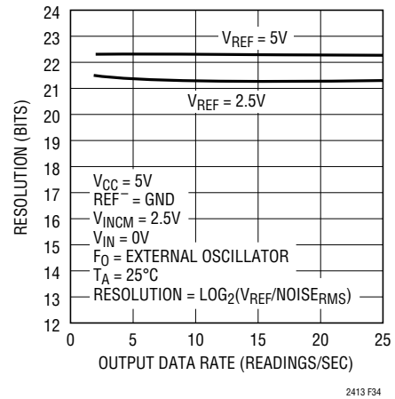
Figure 34. Resolution ( \text{Noise}_{RMS} \leq 1\text{LSB} ) vs Output Data Rate and Reference Voltage
