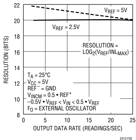
Figure 35. Resolution ( \text{INL}_{MAX} \leq 1\text{LSB} ) vs Output Data Rate and Reference Voltage
