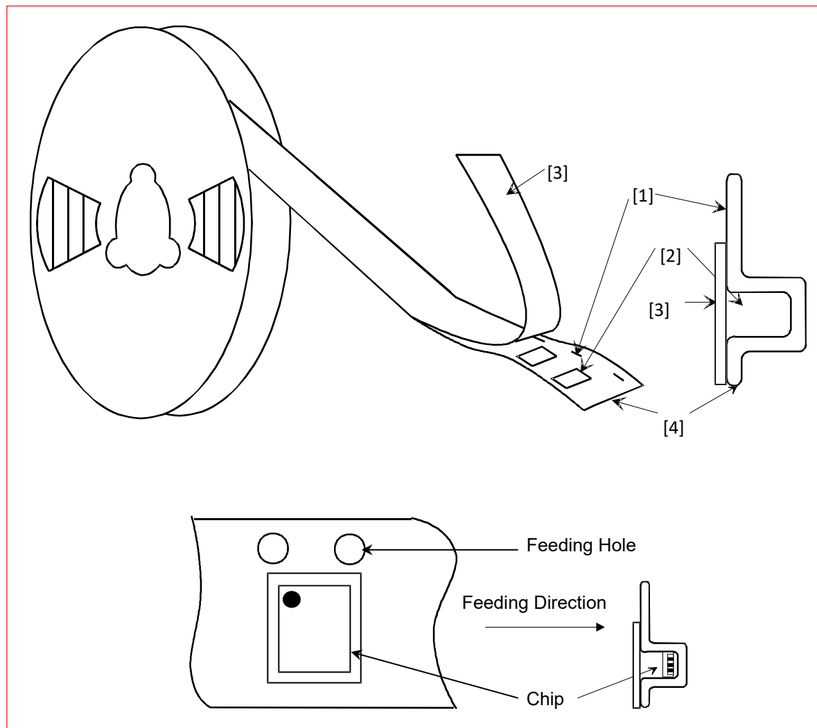
Figure 29: Taping Diagrams
