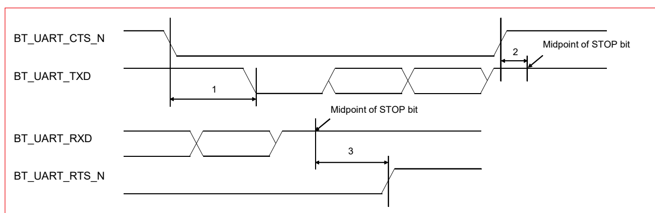
Figure 8: Bluetooth UART Timing Sequence
