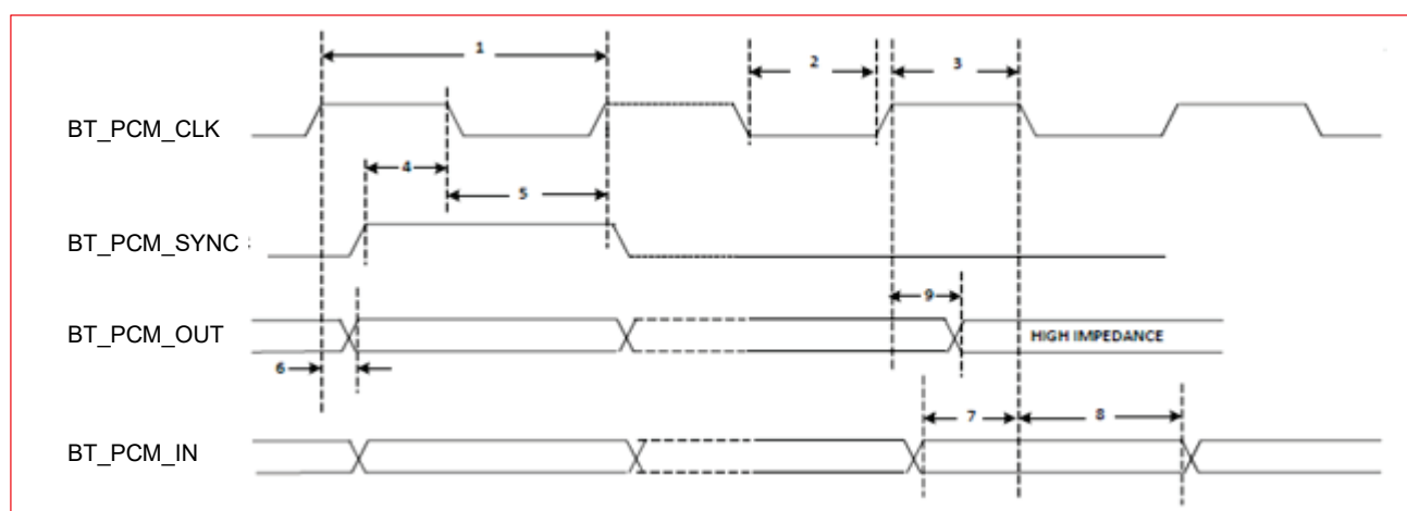
Figure 10: Short Frame Sync Signal - Slave Mode
