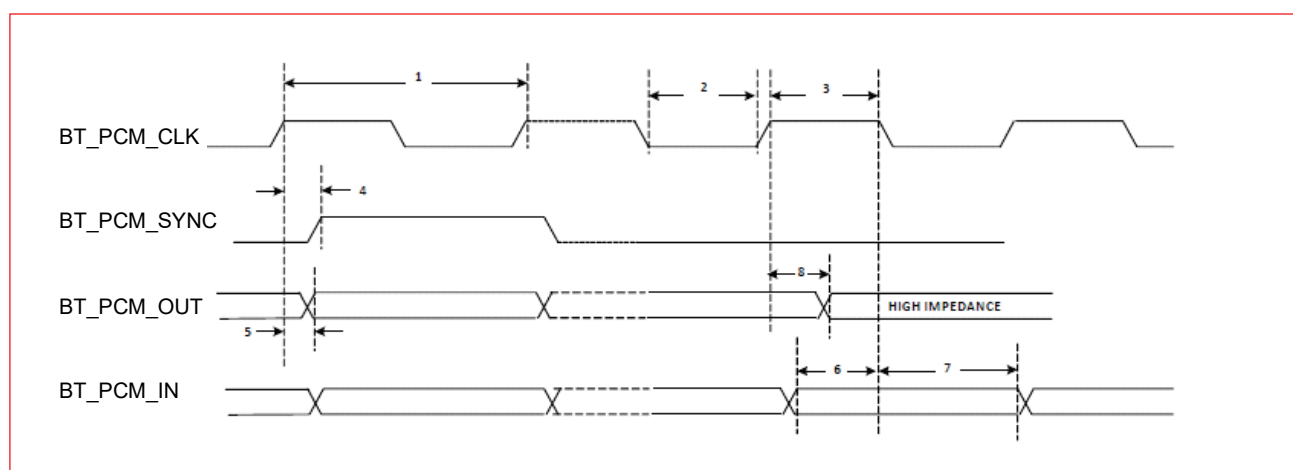
Figure 9: Short Frame Sync Signal - Master Mode
