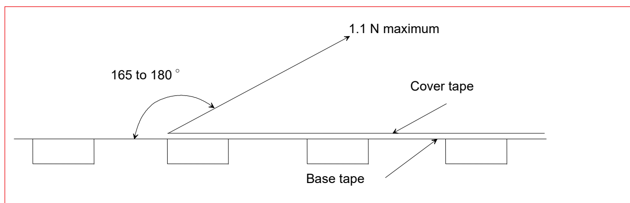
Figure 31: Peeling Force
