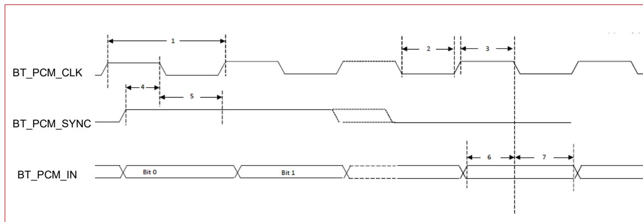
Figure 14: Long Frame Sync Signal - Burst Mode
