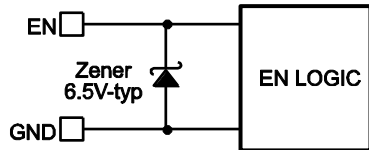
Figure 3: 6.5V Zener Diode Connection
