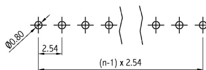
PCB Layouts
