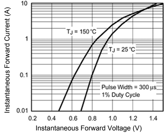
Figure 2. Typical Forward Voltage Characteristics Per Leg
