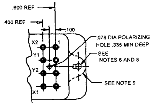
MATING FACE
