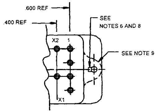
MATING FACE
