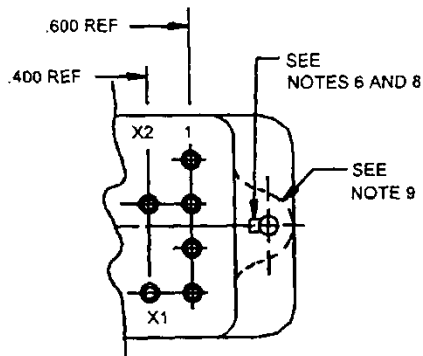
MATING FACE
