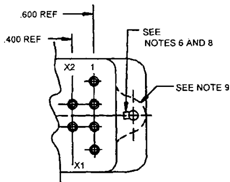
MATING FACE
