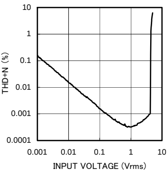
Fig.8 Total Harmonic Distortion - Input Voltage
