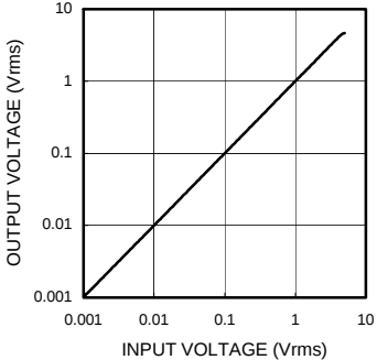
Fig.11 REC Output Voltage - Input Voltage
