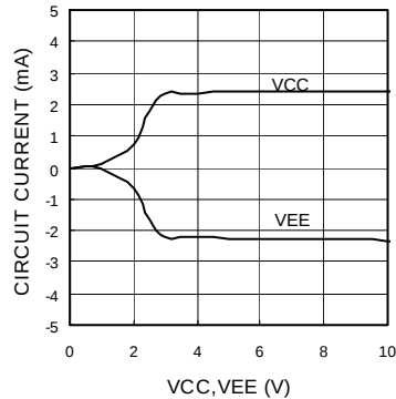
Fig.6 Circuit Current - Supply Voltage
