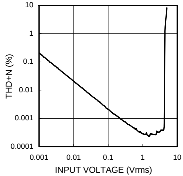
Fig.12 REC Total Harmonic Distortion - Input Voltage
