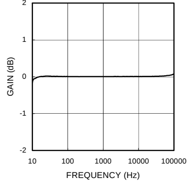
Fig.13 REC Voltage Gain - Frequency
