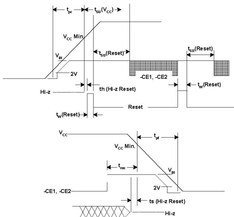
Figure 3: Power Up/Power Down Timing for Systems supporting RESET
