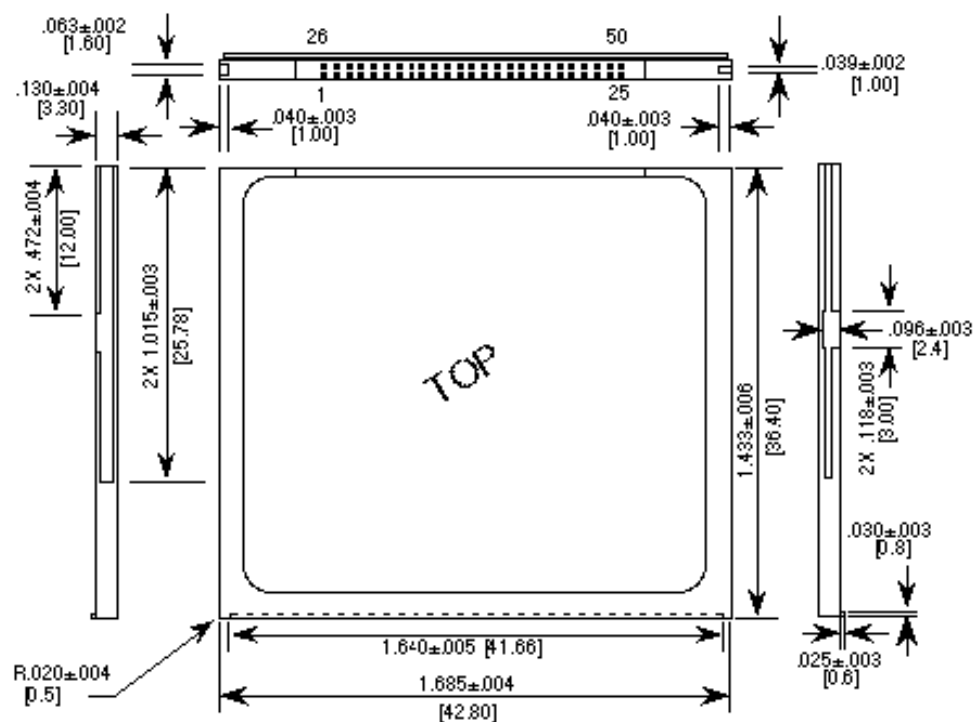
Figure 2: CompactFlash 5000 Dimensions
