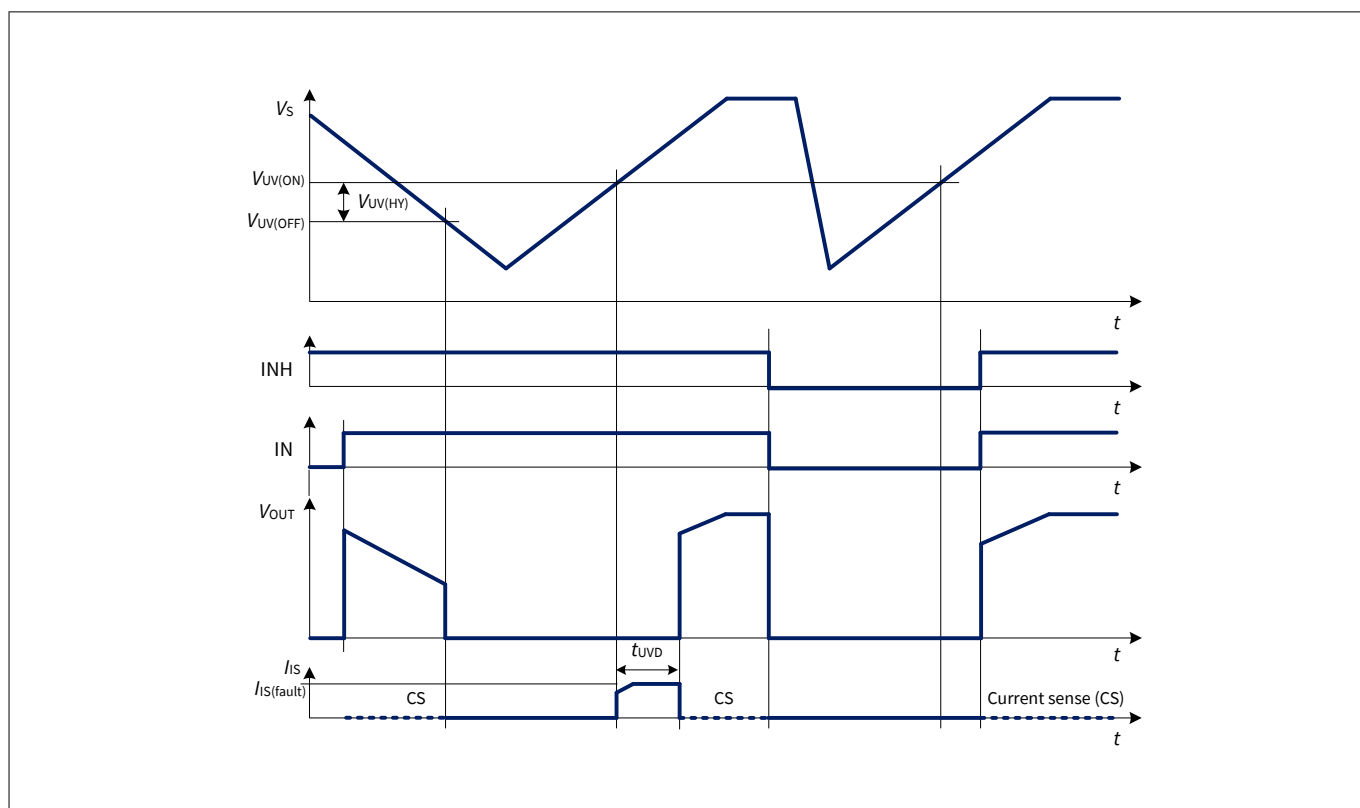
Figure 10 Timing diagram for undervoltage behavior for load to GND
